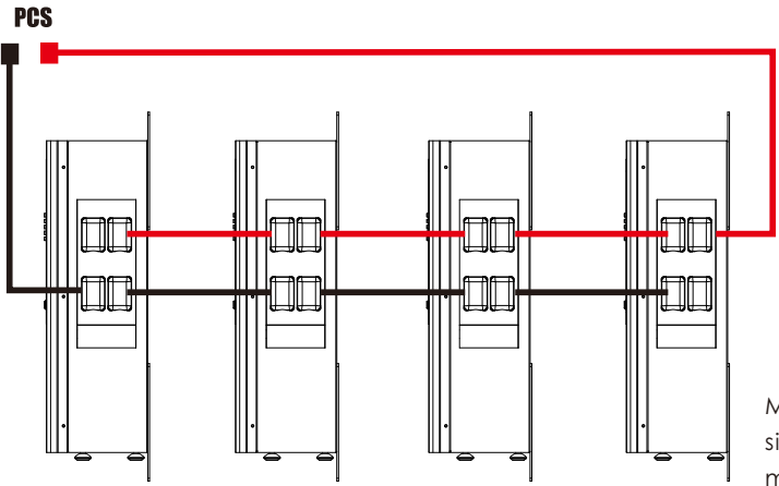
Multi-Units Connection
